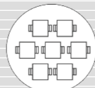
Shell Size 23 Arr. 23-7
