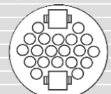
Shell Size 23 Arr. 23-22M
